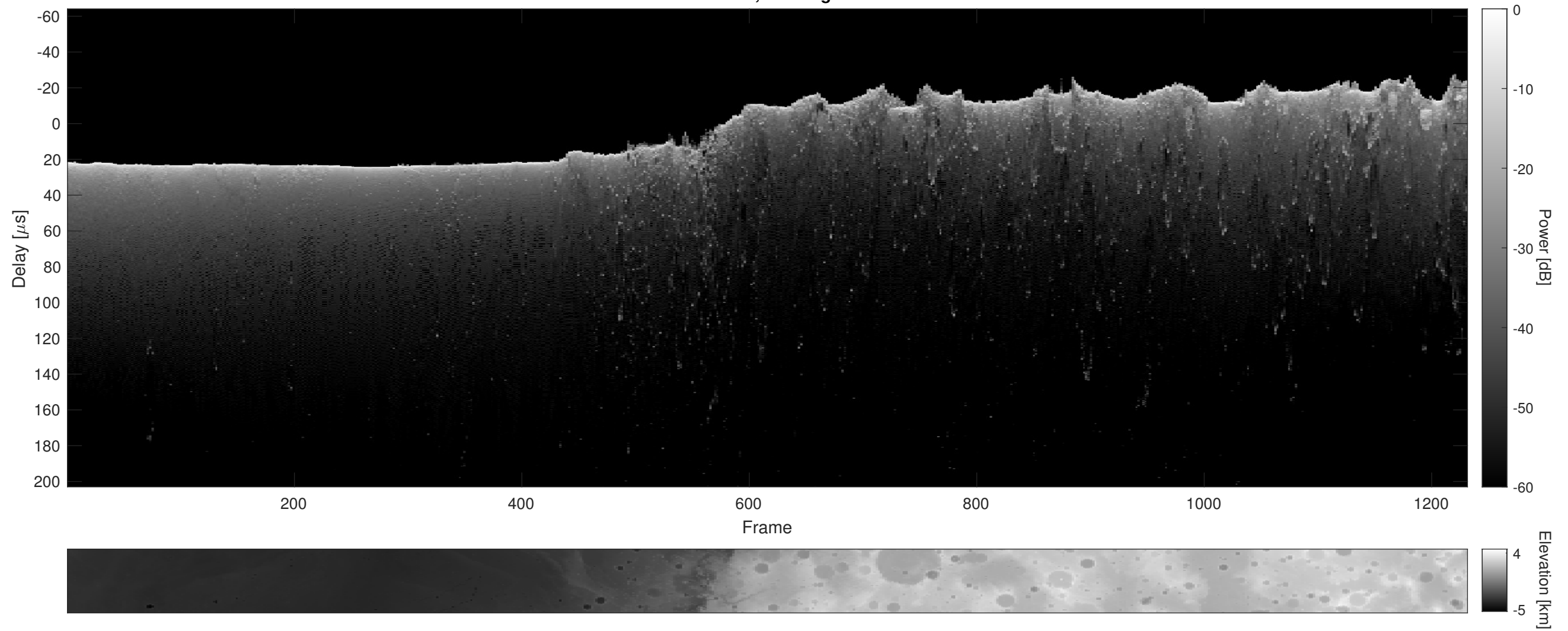
Orbit 5086, Cluttergram
