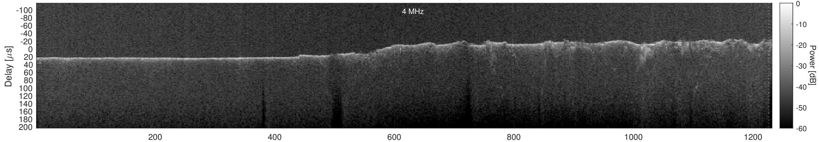
Orbit 5086, Cluttergram
