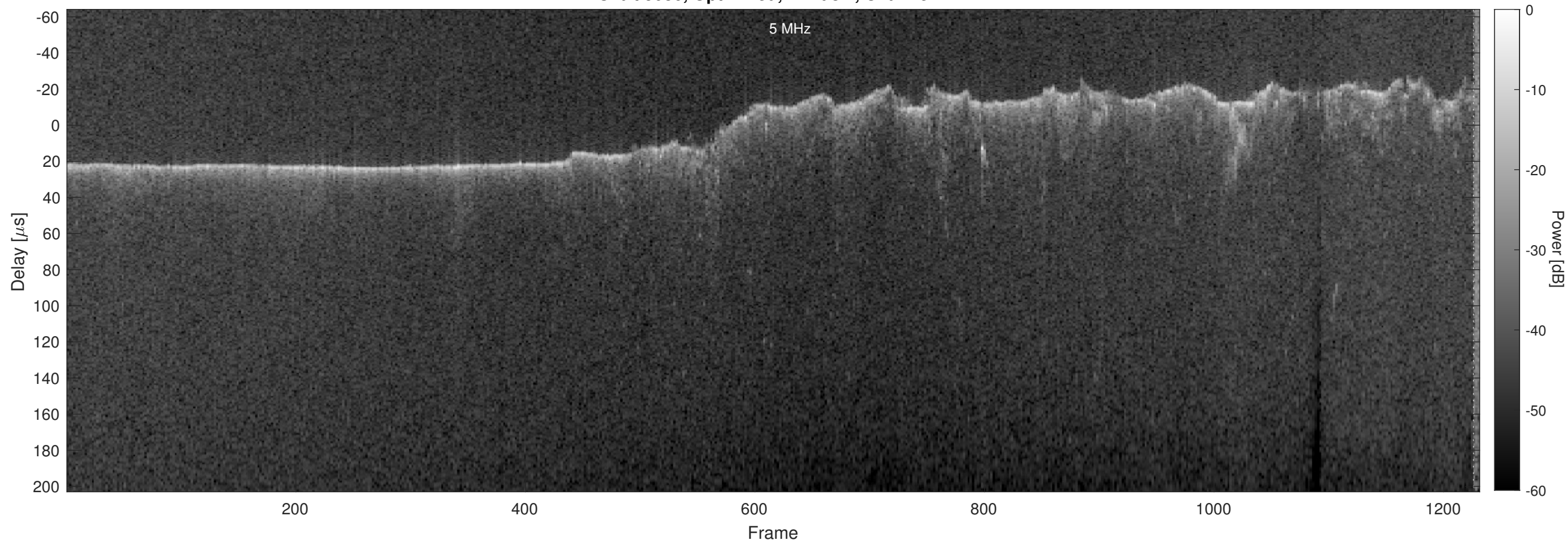
Orbit 5086, Optimized, Window, Channel 2
