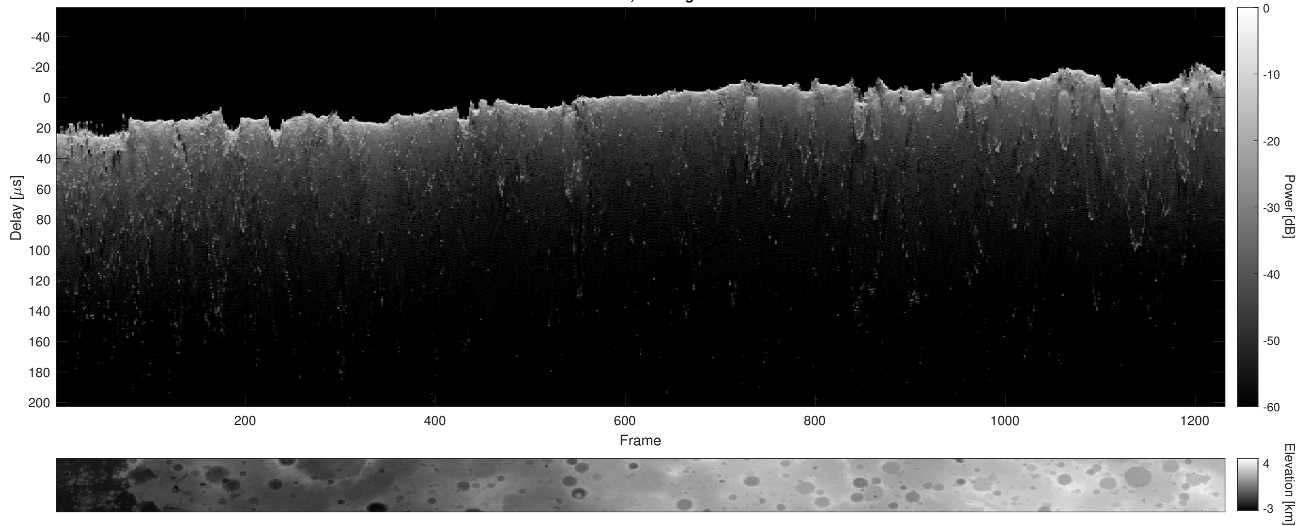
Orbit 5087, Cluttergram
