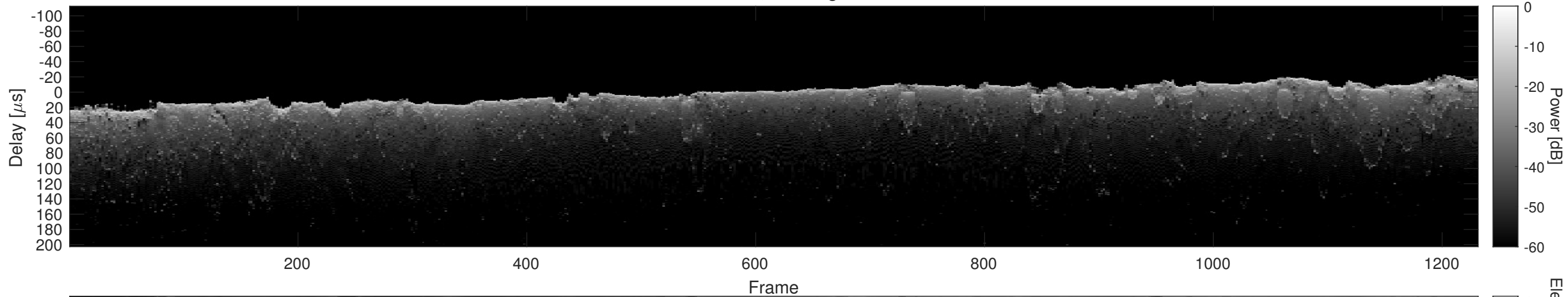
Orbit 5087, Cluttergram
