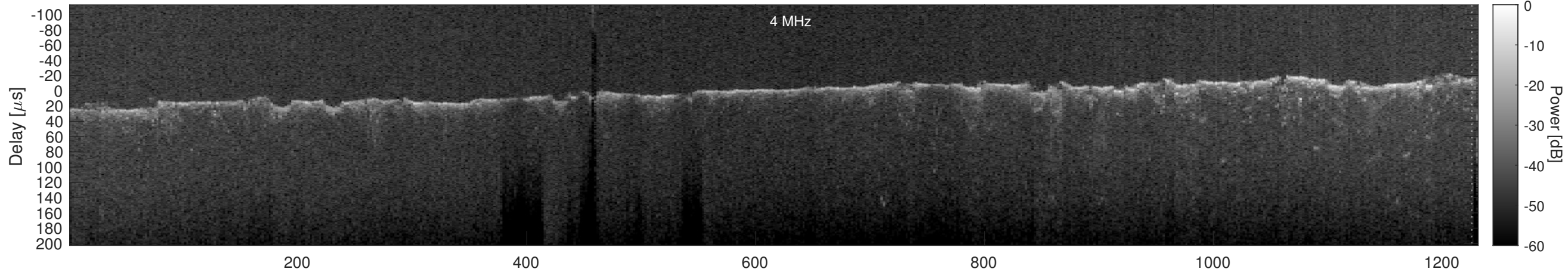
Orbit 5087, Cluttergram
