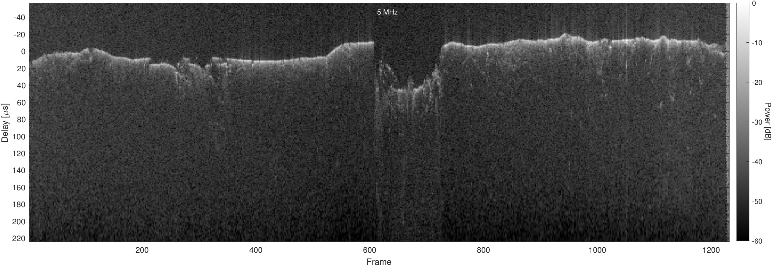
Orbit 5088, Optimized, Window, Channel 2
