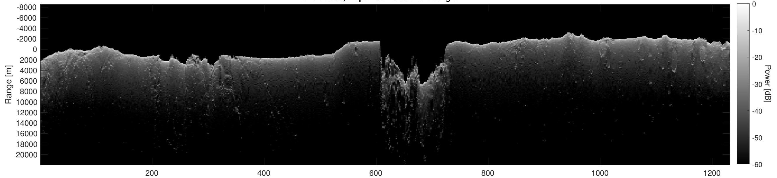
Orbit 5088, Depth-Corrected Cluttergram
