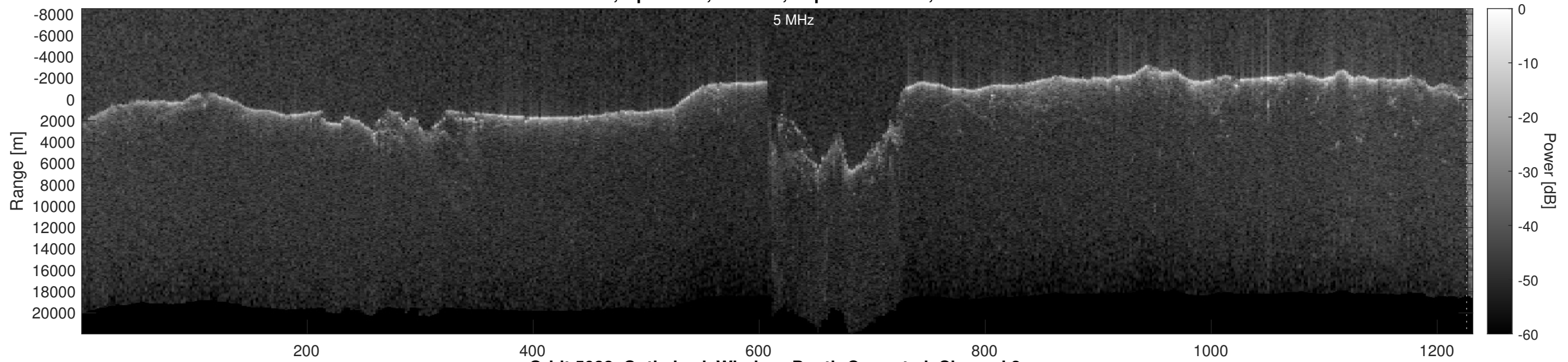
Orbit 5088, Optimized, Window, Depth-Corrected, Channel 2
