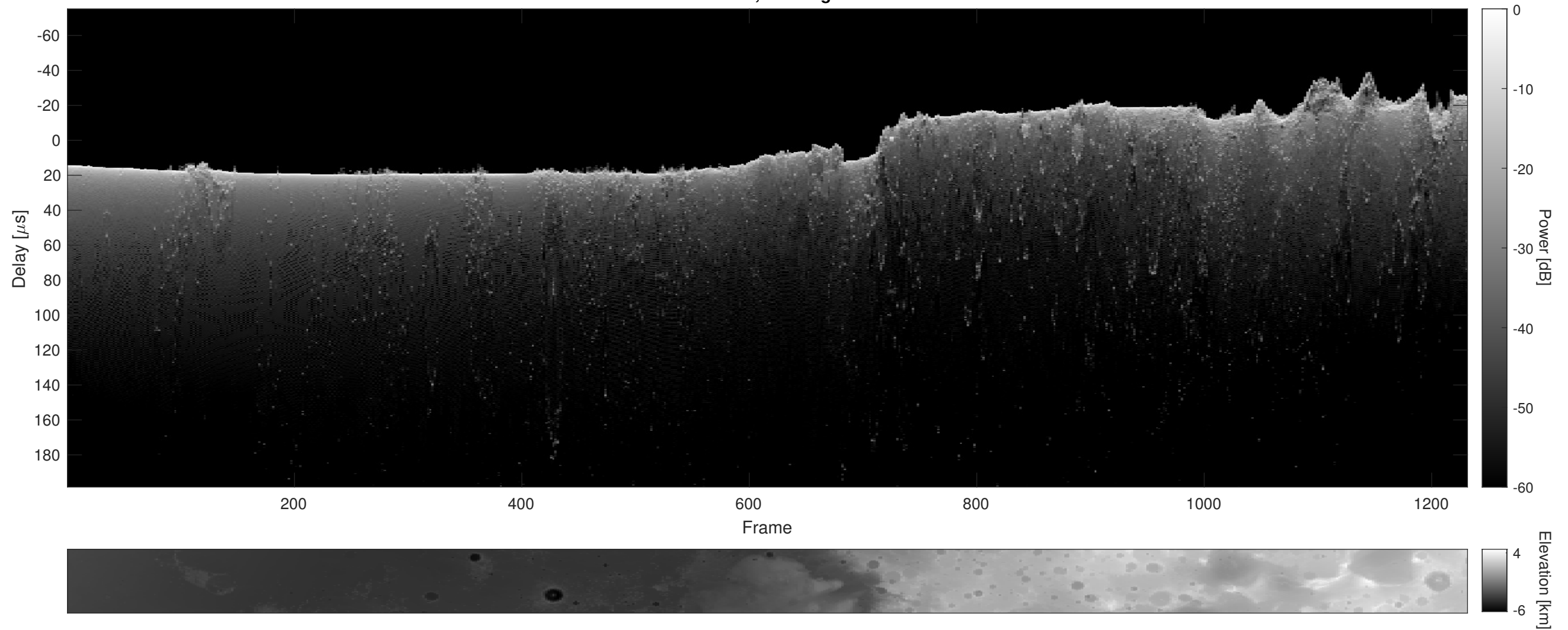
Orbit 5089, Cluttergram
