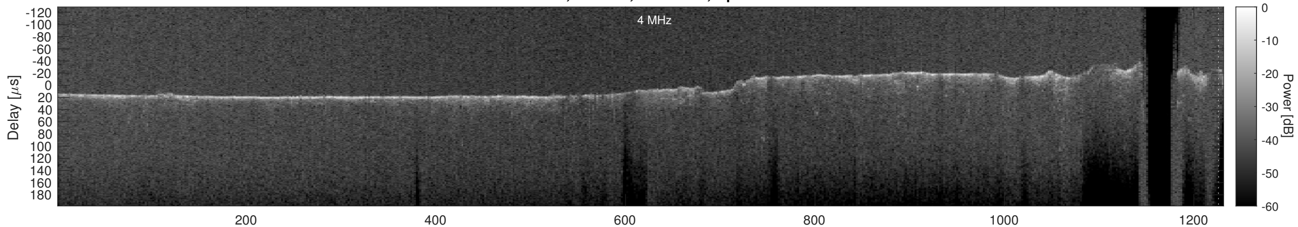
Orbit 5089, Cluttergram
