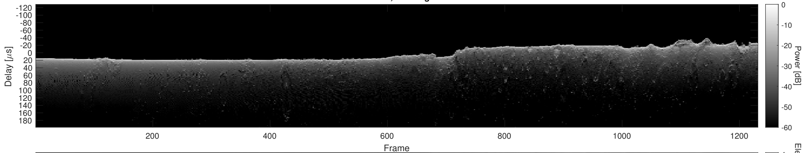
Orbit 5089, Cluttergram
