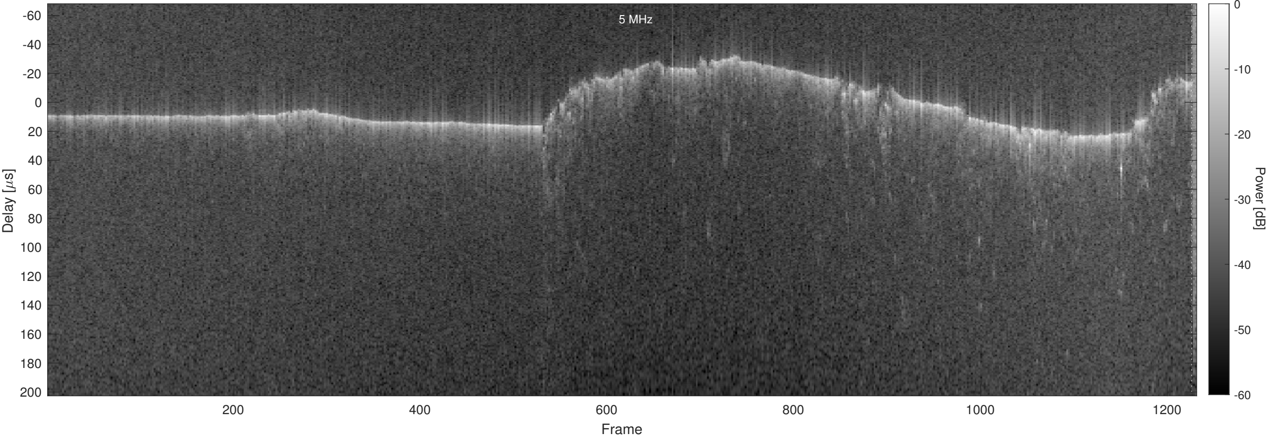
Orbit 5090, Optimized, No Window, Channel 2
