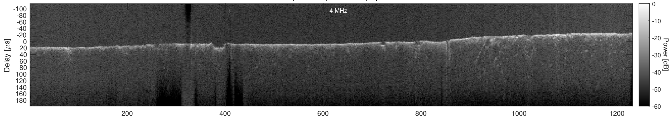
Orbit 5091, Cluttergram
