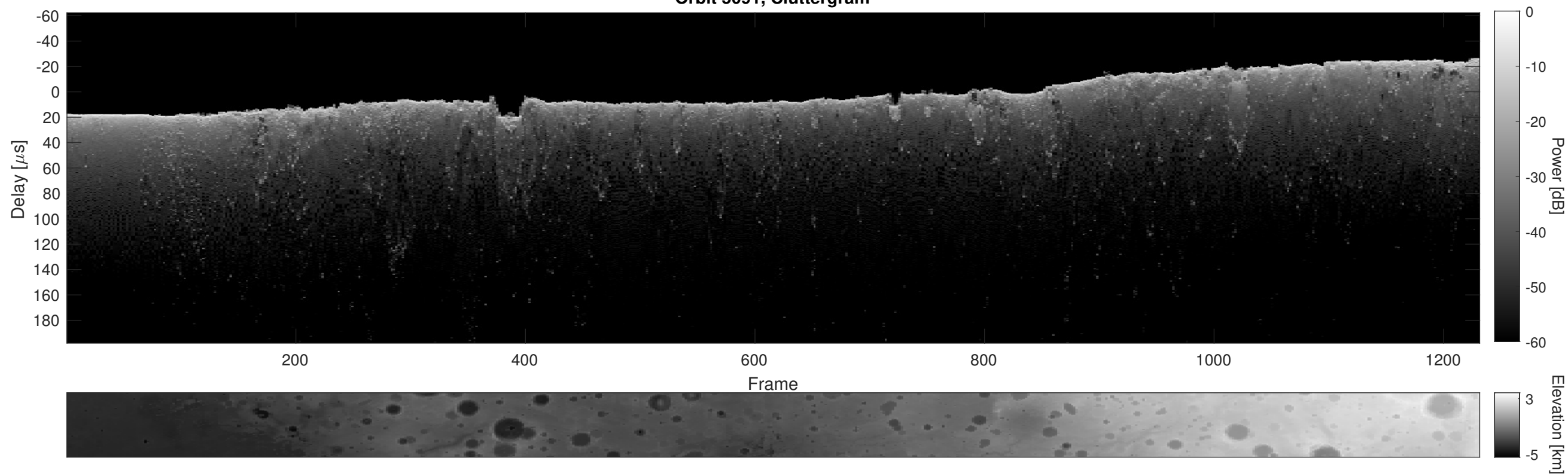
Orbit 5091, Cluttergram
