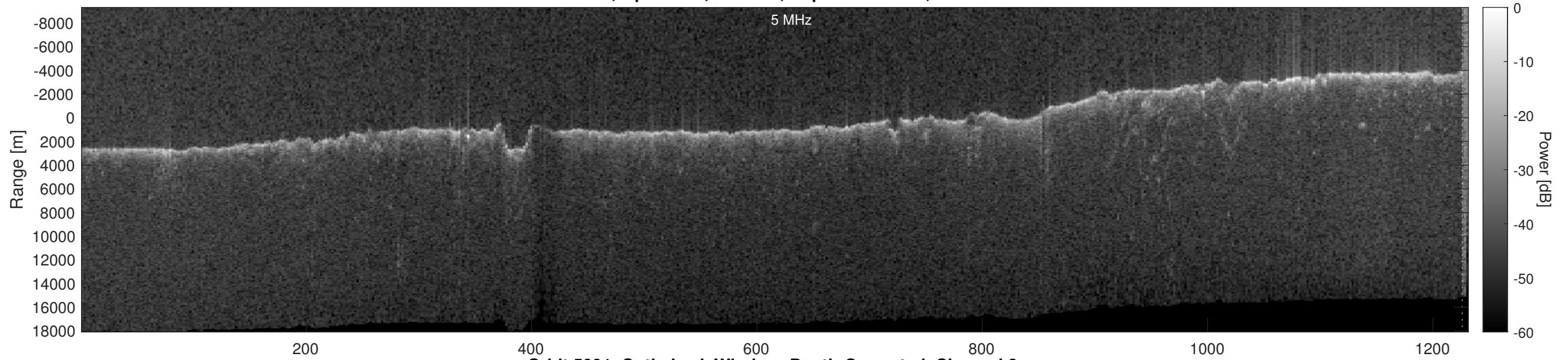
Orbit 5091, Optimized, Window, Depth-Corrected, Channel 2
