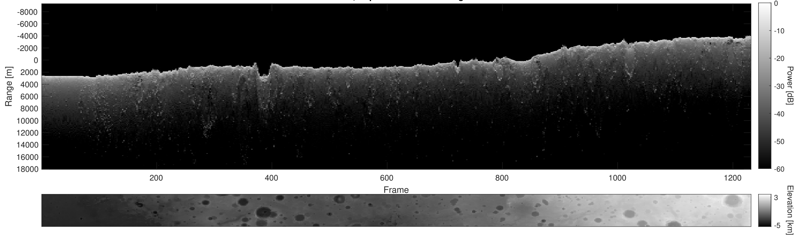
Orbit 5091, Depth-Corrected Cluttergram
