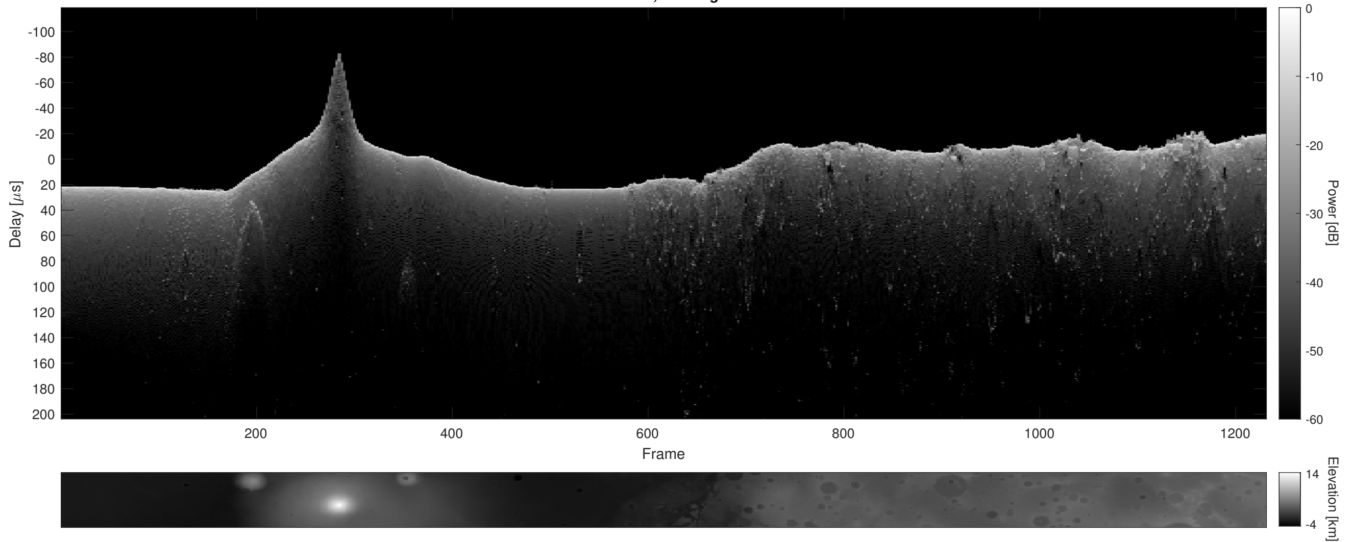
Orbit 5093, Cluttergram
