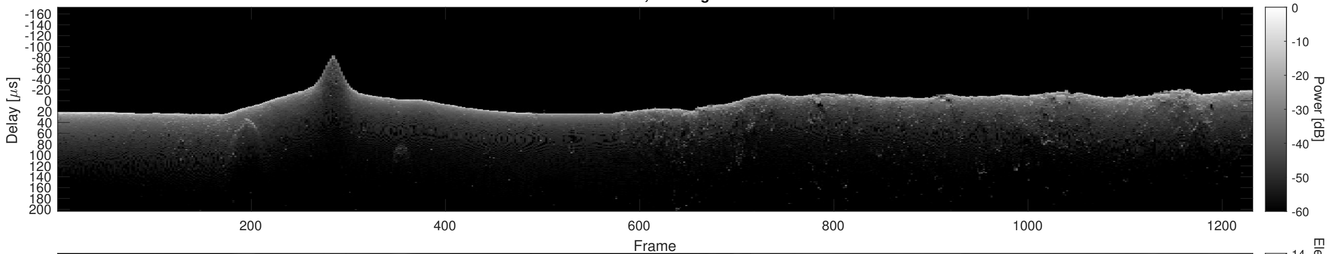
Orbit 5093, Cluttergram
