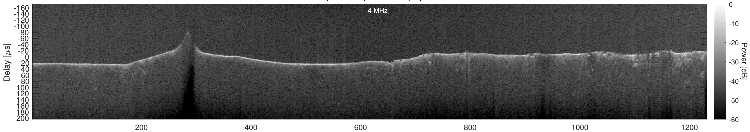
Orbit 5093, Cluttergram
