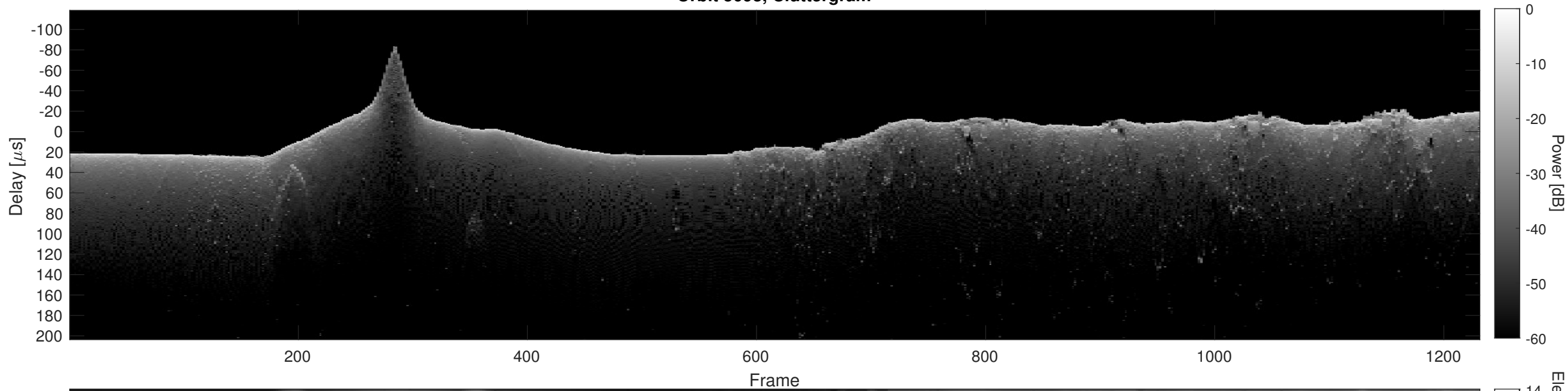
Orbit 5093, Cluttergram
