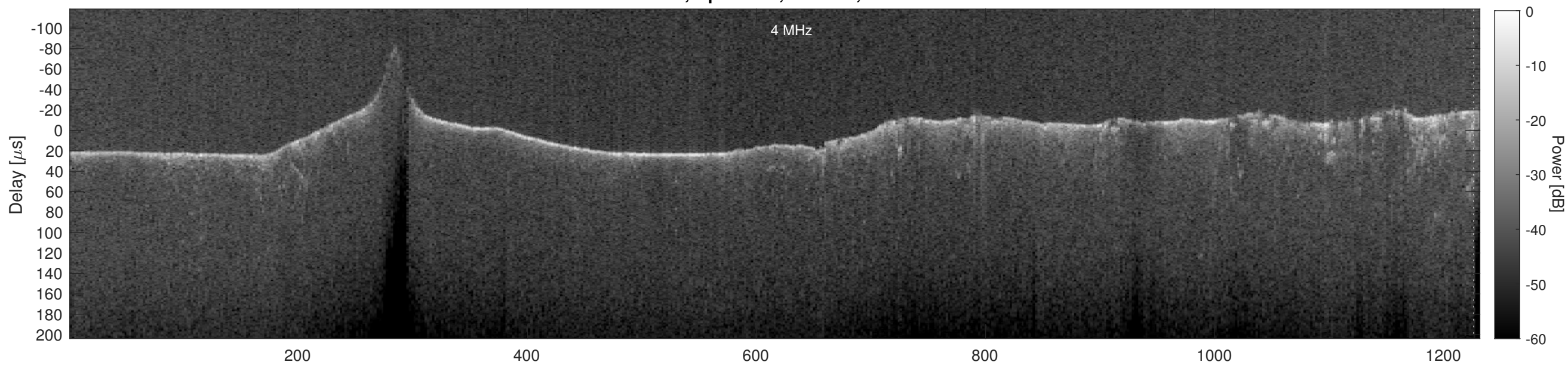
Orbit 5093, Cluttergram
