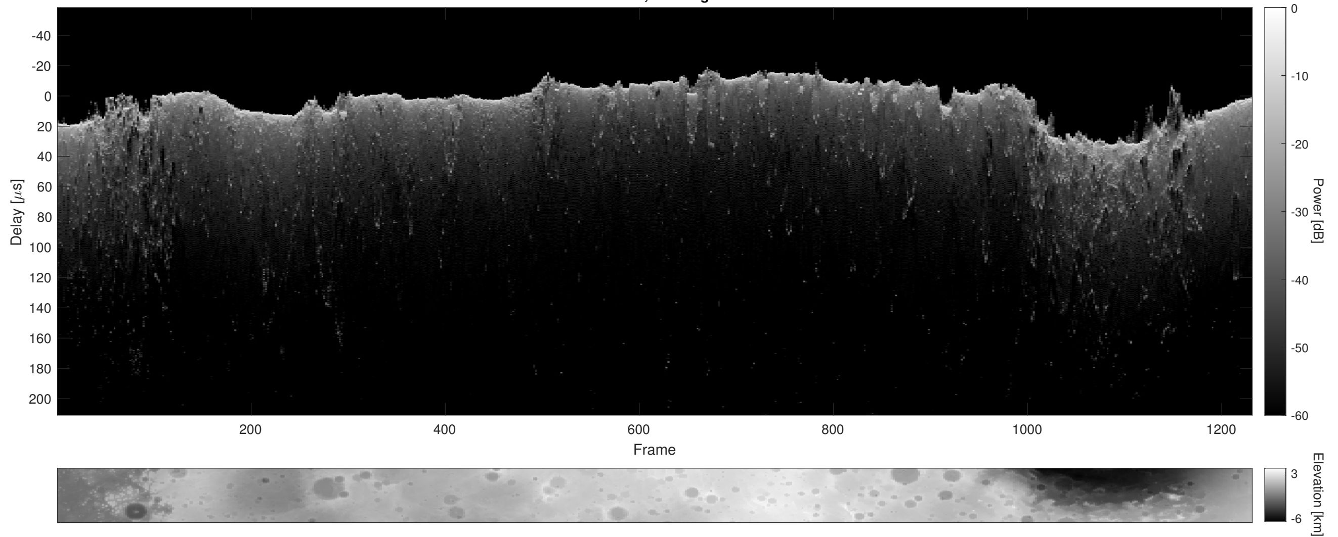
Orbit 5094, Cluttergram
