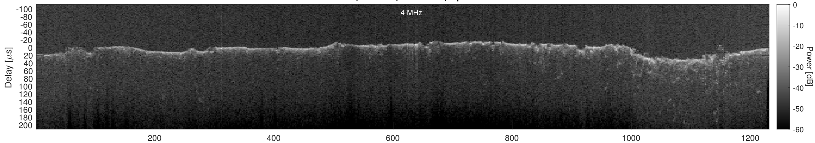
Orbit 5094, Cluttergram
