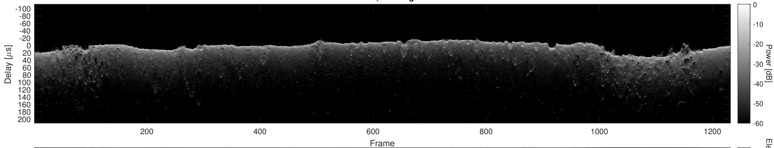
Orbit 5094, Cluttergram
