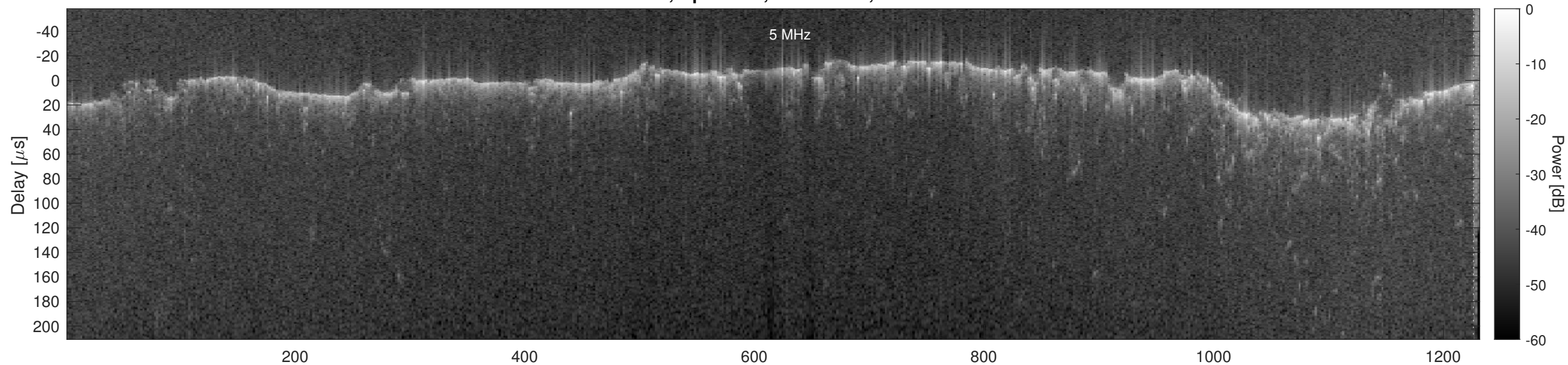
Orbit 5094, Optimized, No Window, Channel 2
