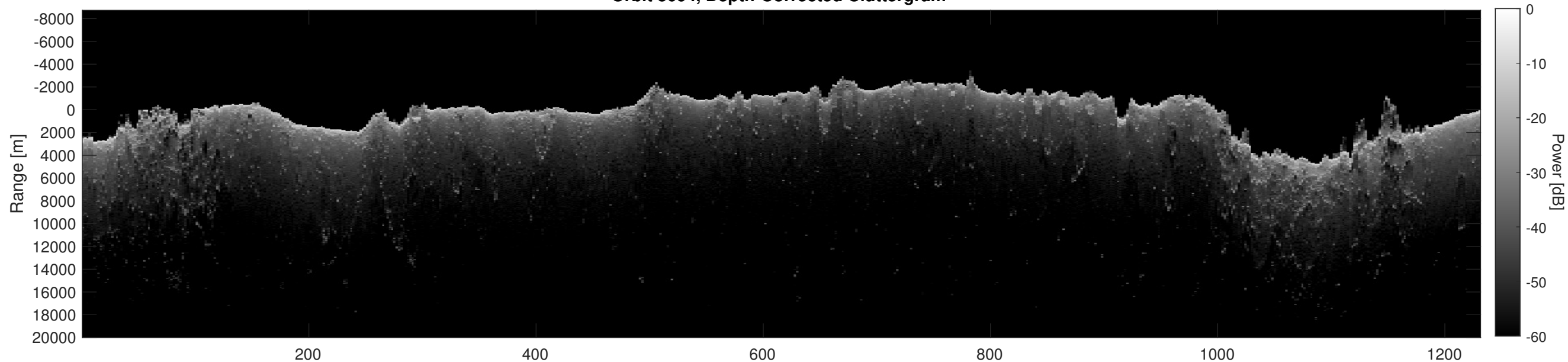
Orbit 5094, Depth-Corrected Cluttergram
