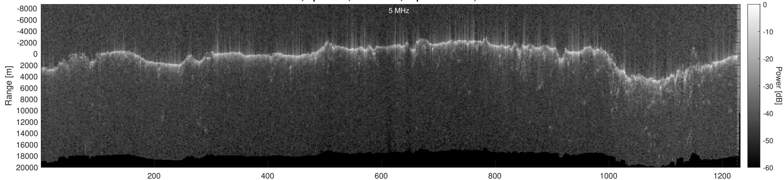
Orbit 5094, Optimized, No Window, Depth-Corrected, Channel 2
