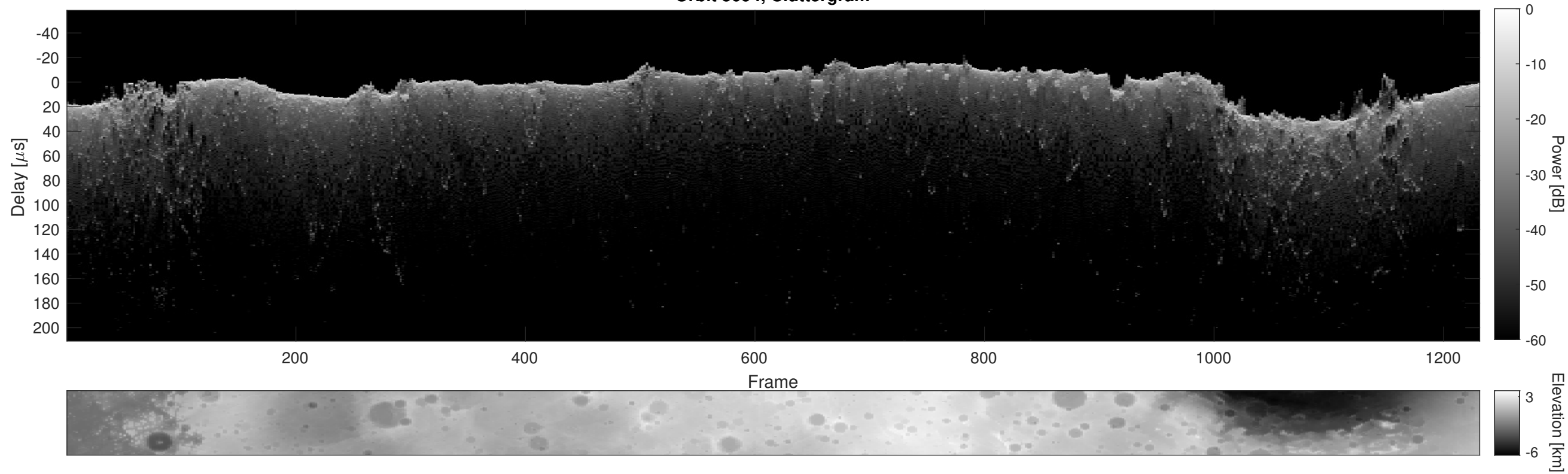
Orbit 5094, Cluttergram
