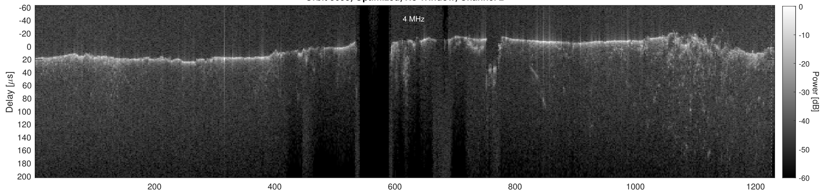
Orbit 5095, Cluttergram
