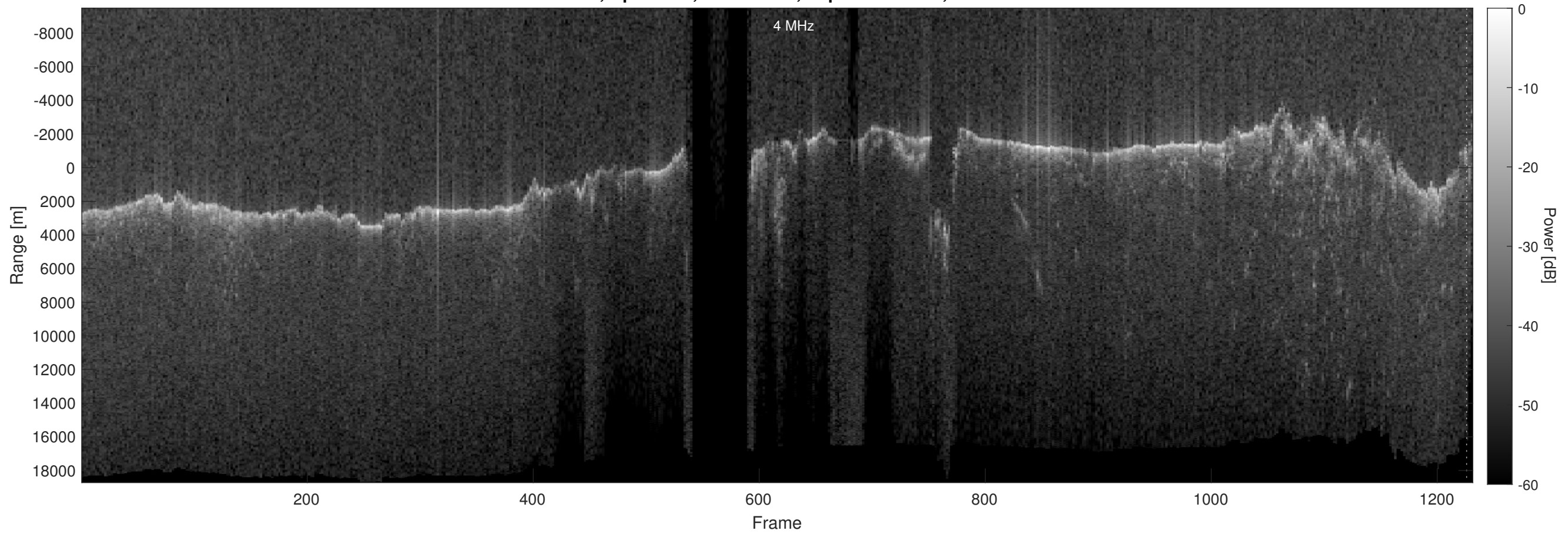
Orbit 5095, Optimized, No Window, Depth-Corrected, Channel 2
