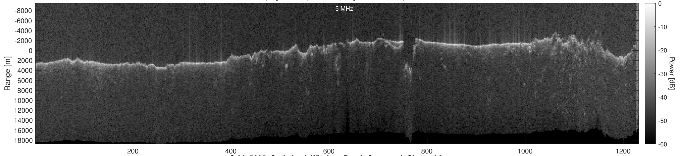
Orbit 5095, Optimized, Window, Depth-Corrected, Channel 2
