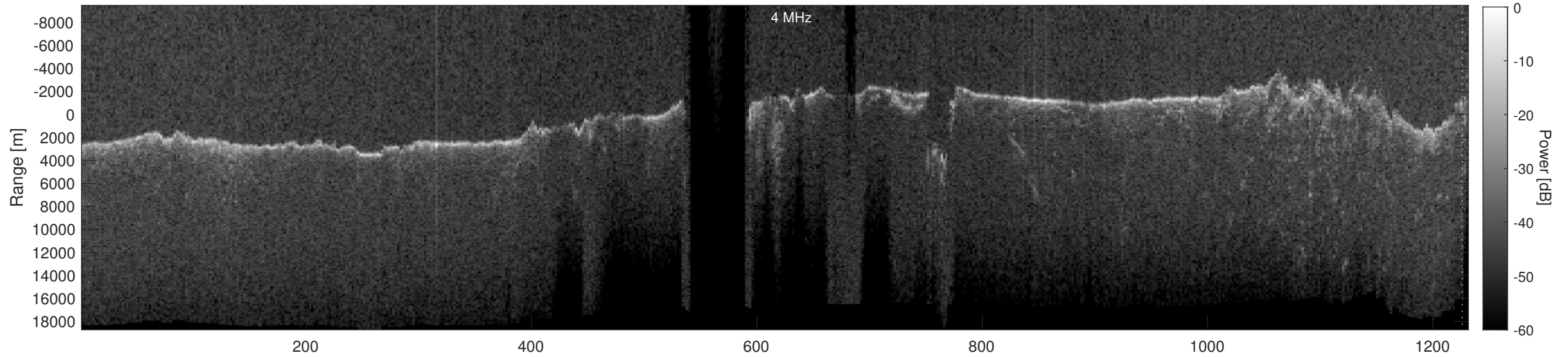
Orbit 5095, Depth-Corrected Cluttergram
