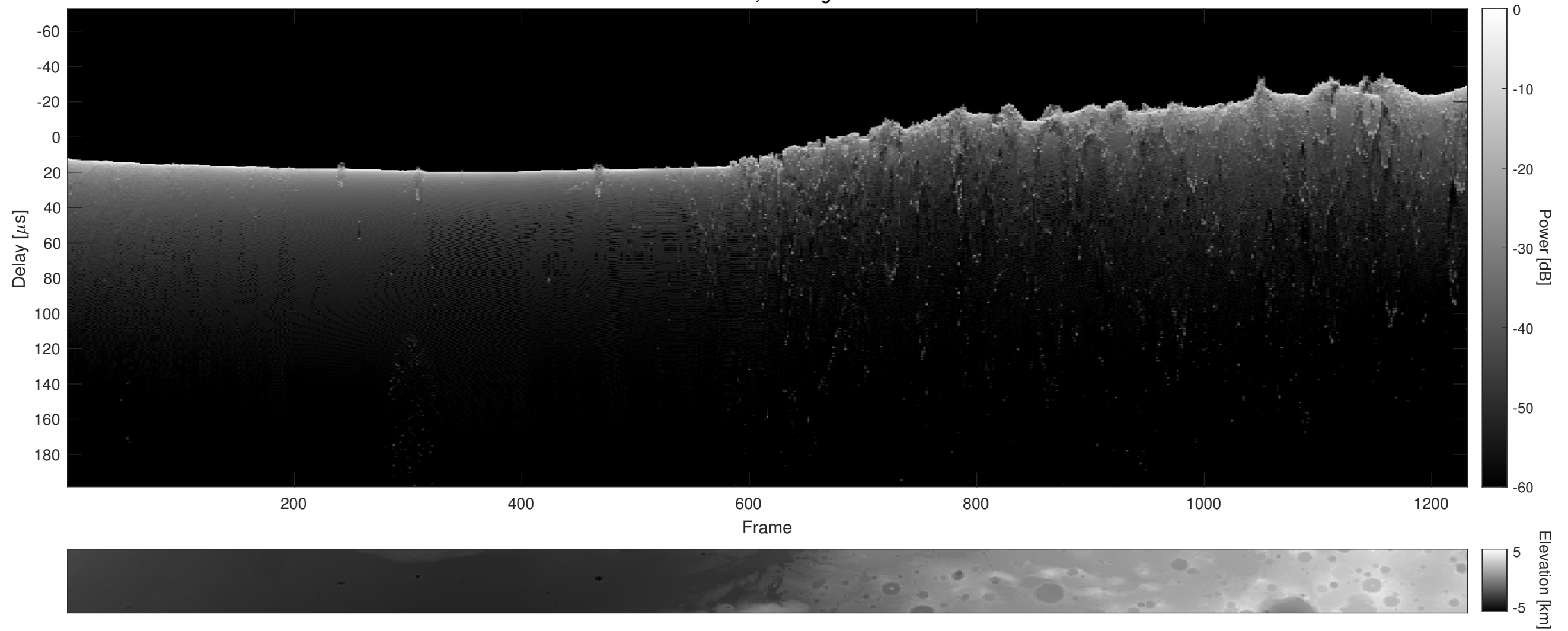
Orbit 5096, Cluttergram
