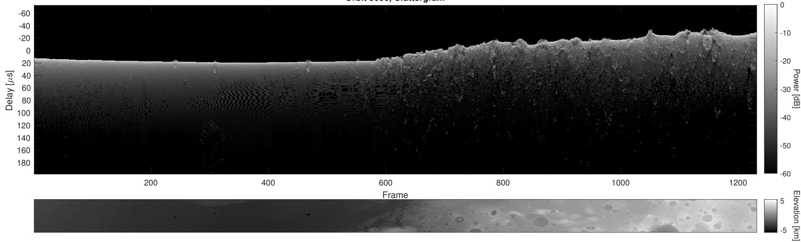
Orbit 5096, Cluttergram
