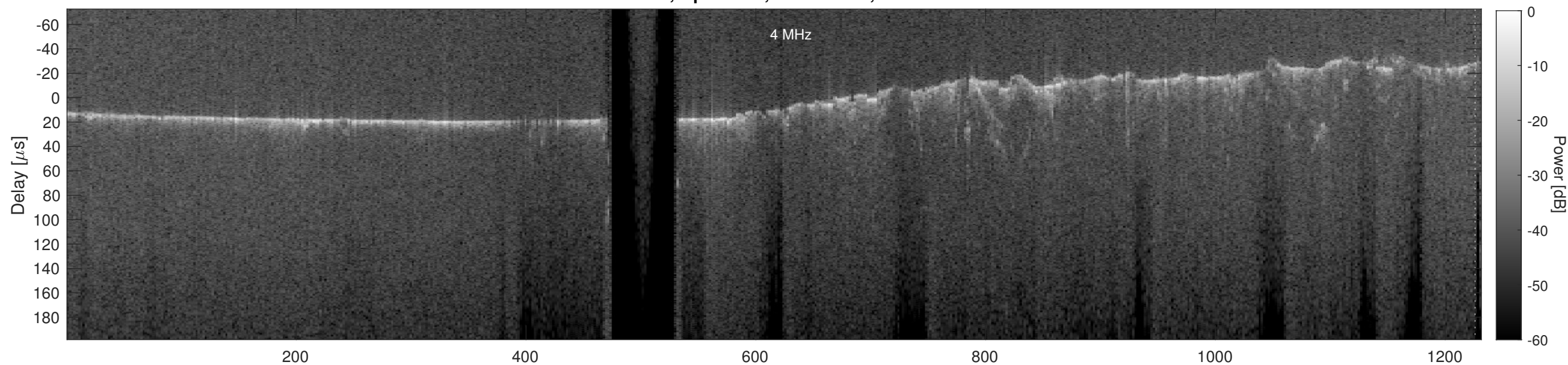
Orbit 5096, Cluttergram
