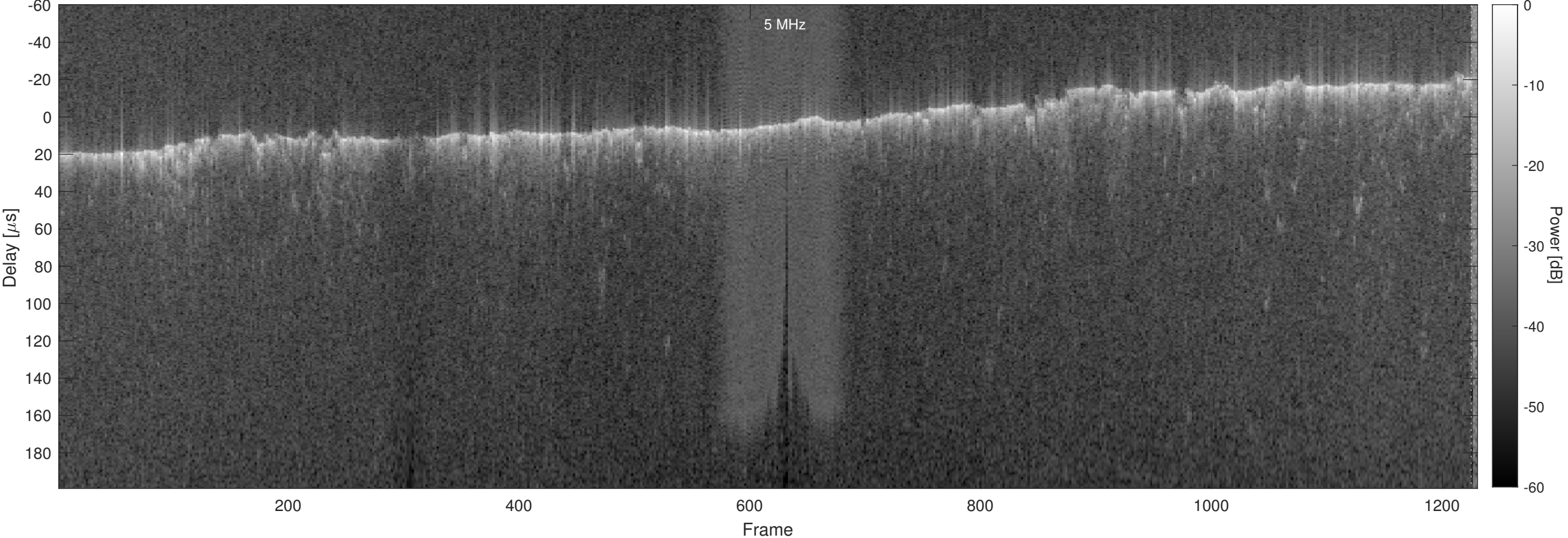
Orbit 5098, Optimized, No Window, Channel 2
