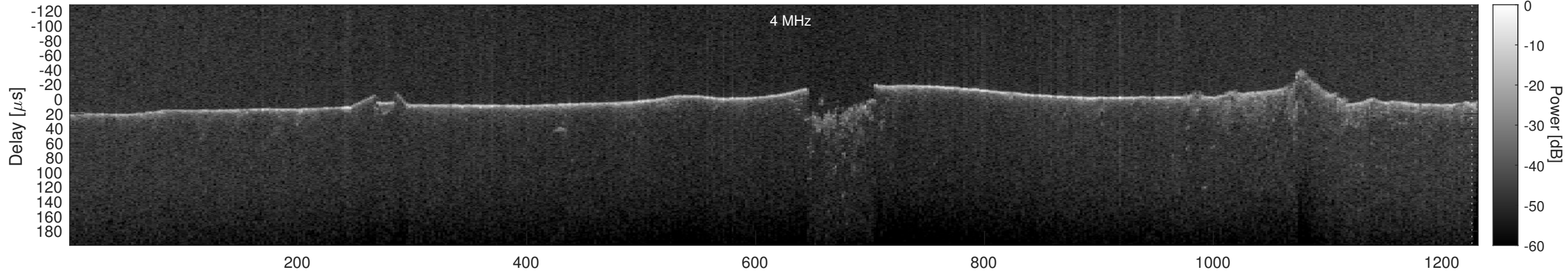
Orbit 5099, Cluttergram
