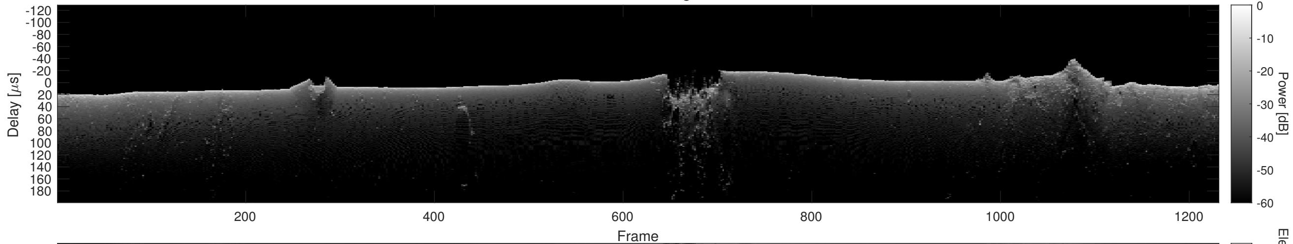
Orbit 5099, Cluttergram
