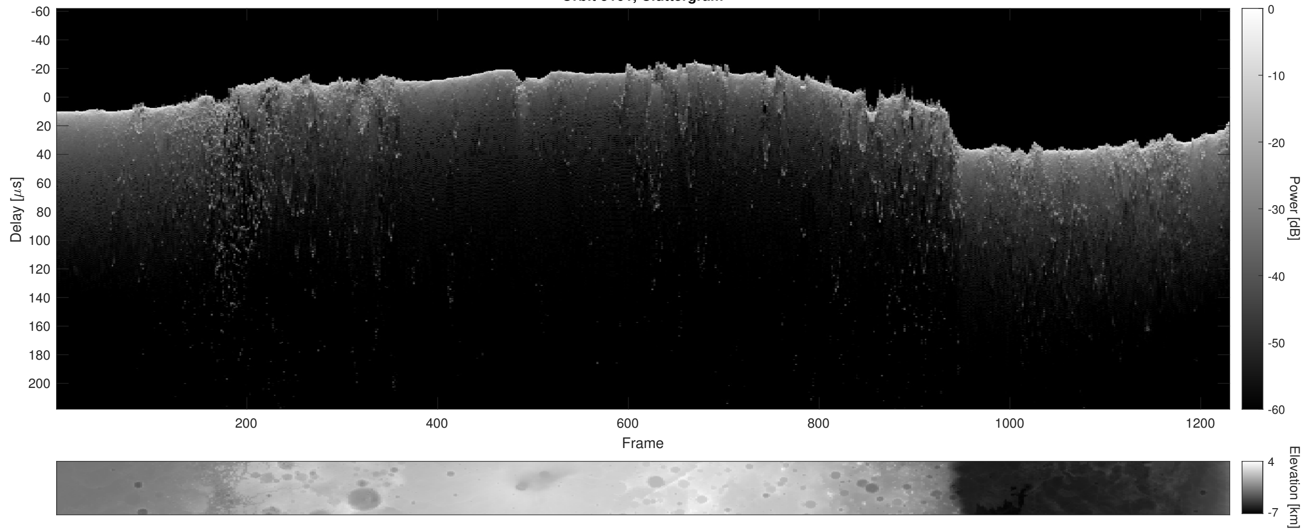
Orbit 5101, Cluttergram
