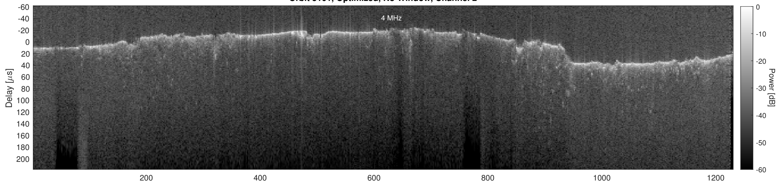
Orbit 5101, Cluttergram
