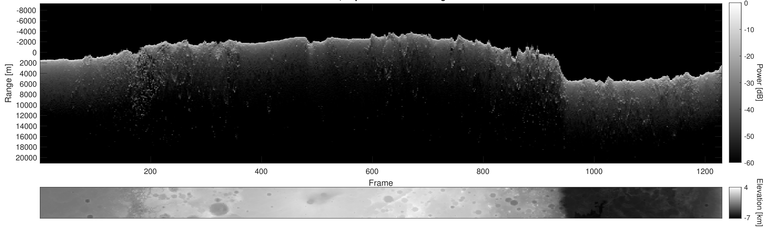
Orbit 5101, Depth-Corrected Cluttergram
