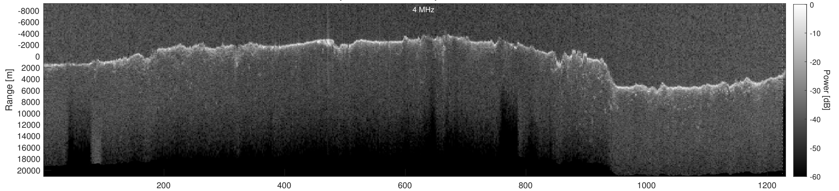
Orbit 5101, Depth-Corrected Cluttergram
