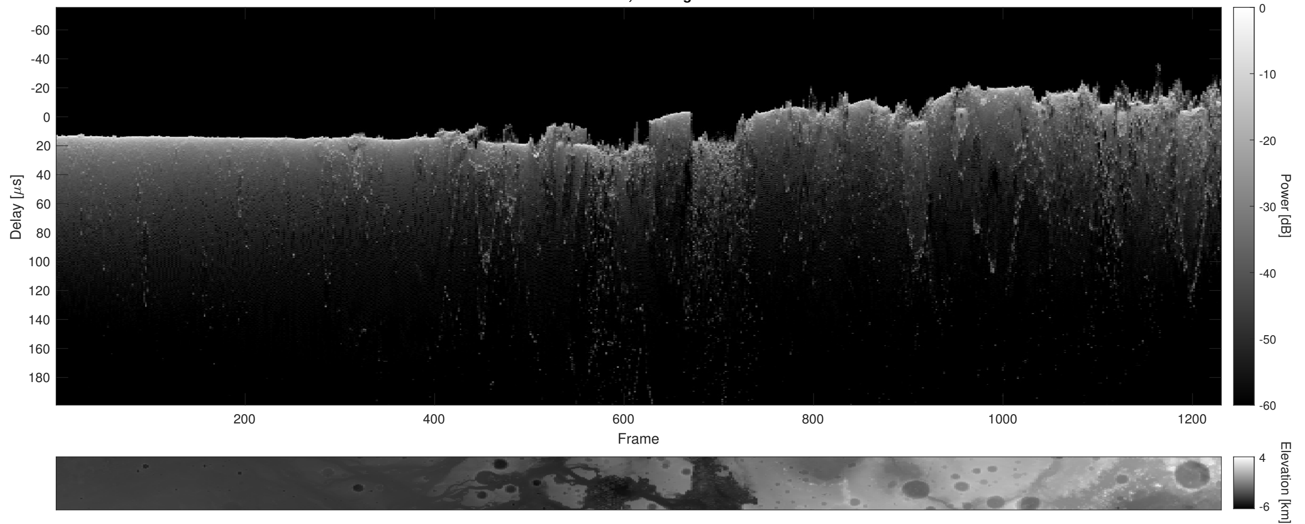
Orbit 5102, Cluttergram
