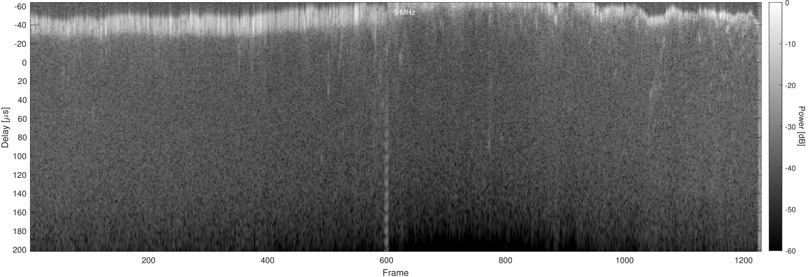
Orbit 5104, Chapman, Window, Channel 2
