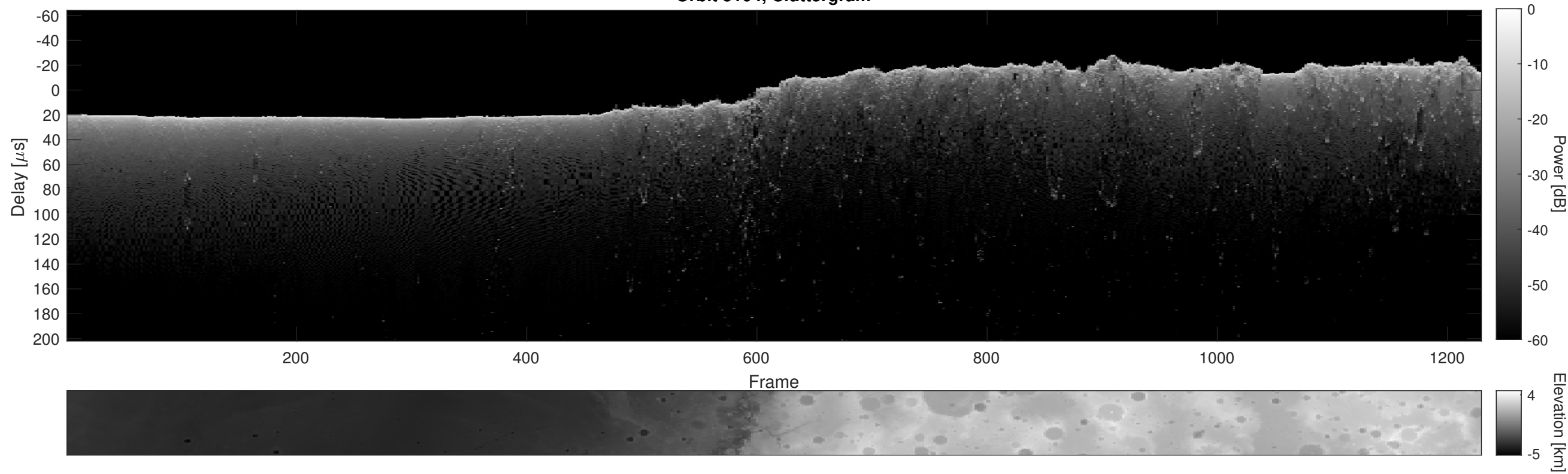
Orbit 5104, Cluttergram
