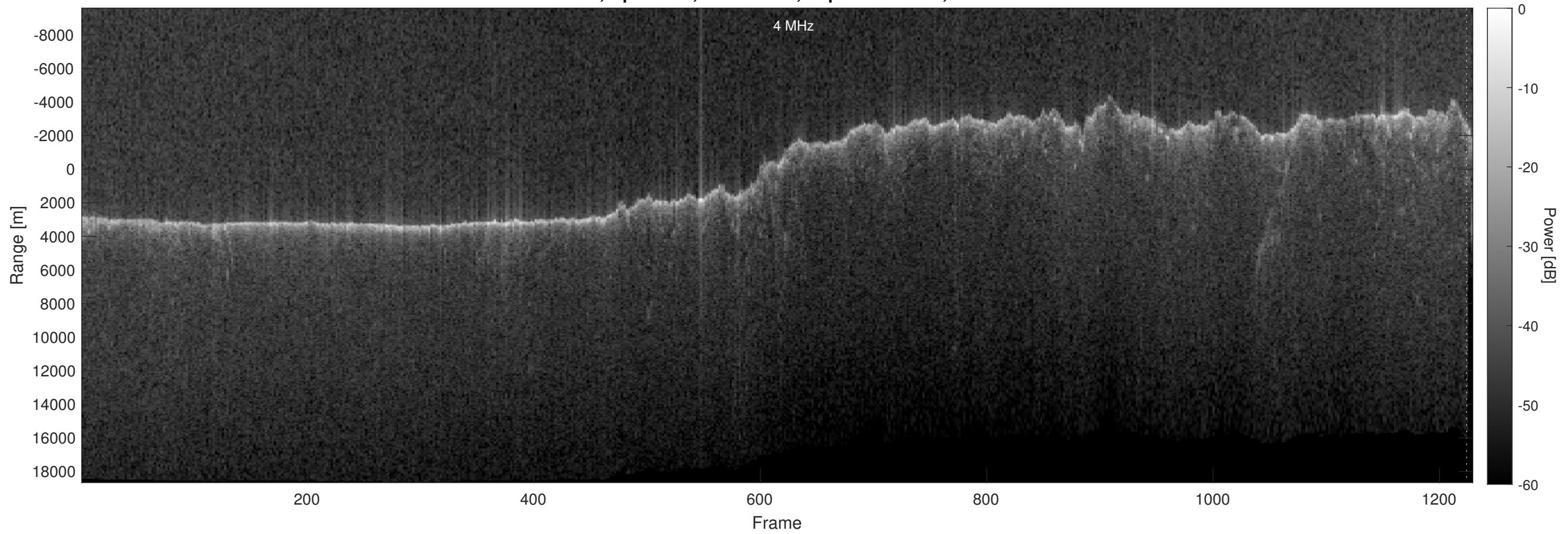
Orbit 5104, Optimized, No Window, Depth-Corrected, Channel 2
