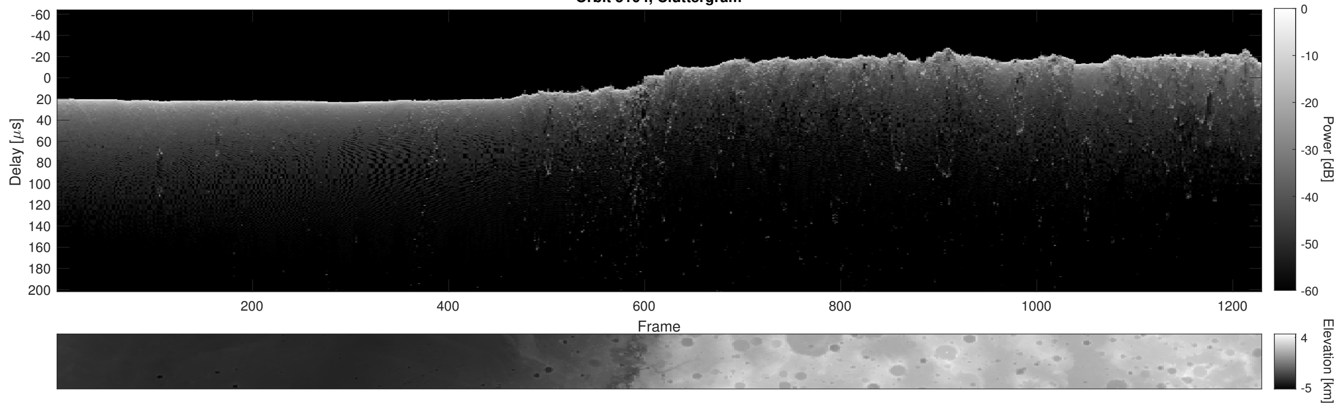
Orbit 5104, Cluttergram
