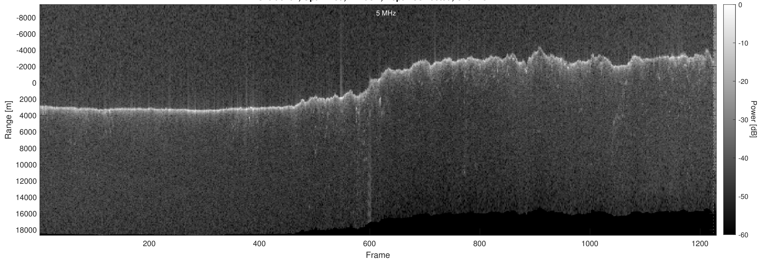
Orbit 5104, Optimized, Window, Depth-Corrected, Channel 2
