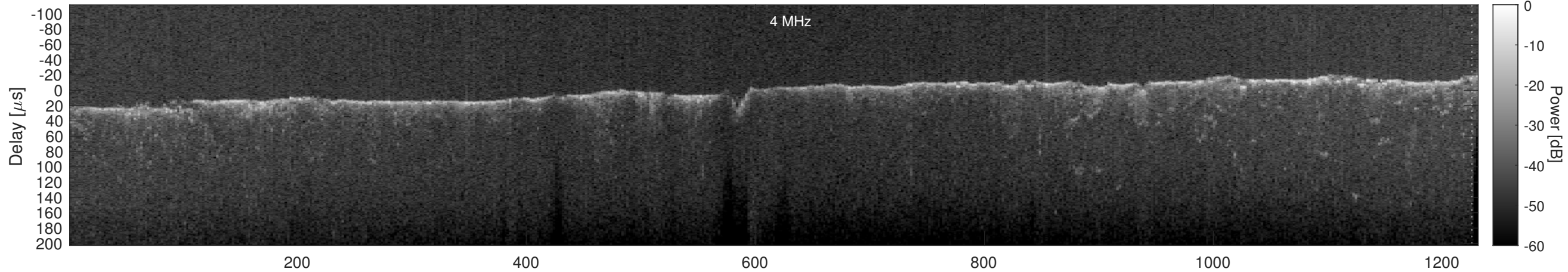
Orbit 5105, Cluttergram
