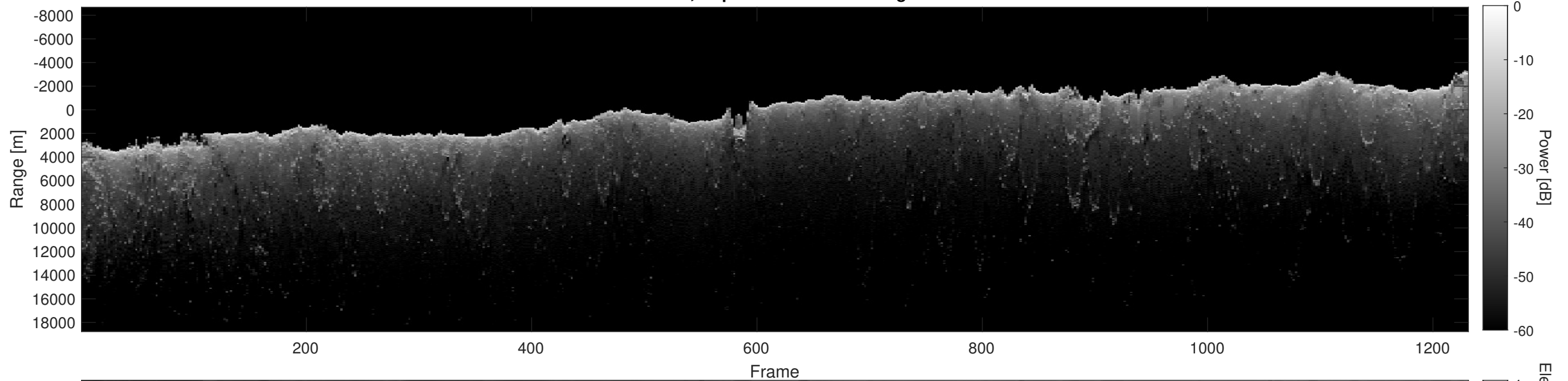
Orbit 5105, Depth-Corrected Cluttergram
