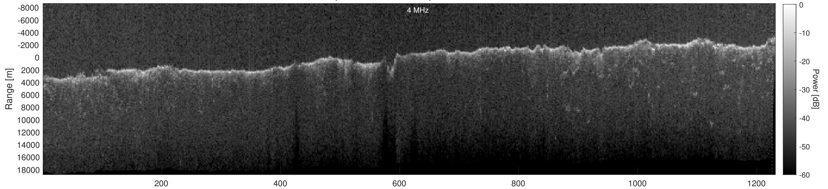
Orbit 5105, Depth-Corrected Cluttergram
