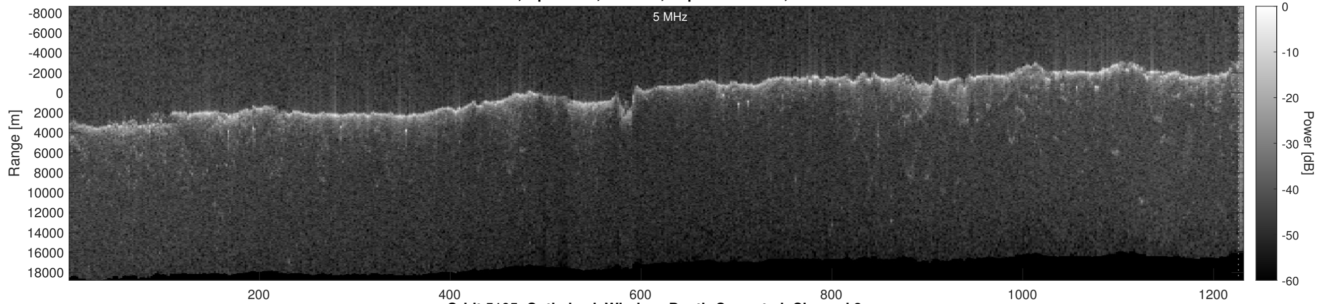
Orbit 5105, Optimized, Window, Depth-Corrected, Channel 2
