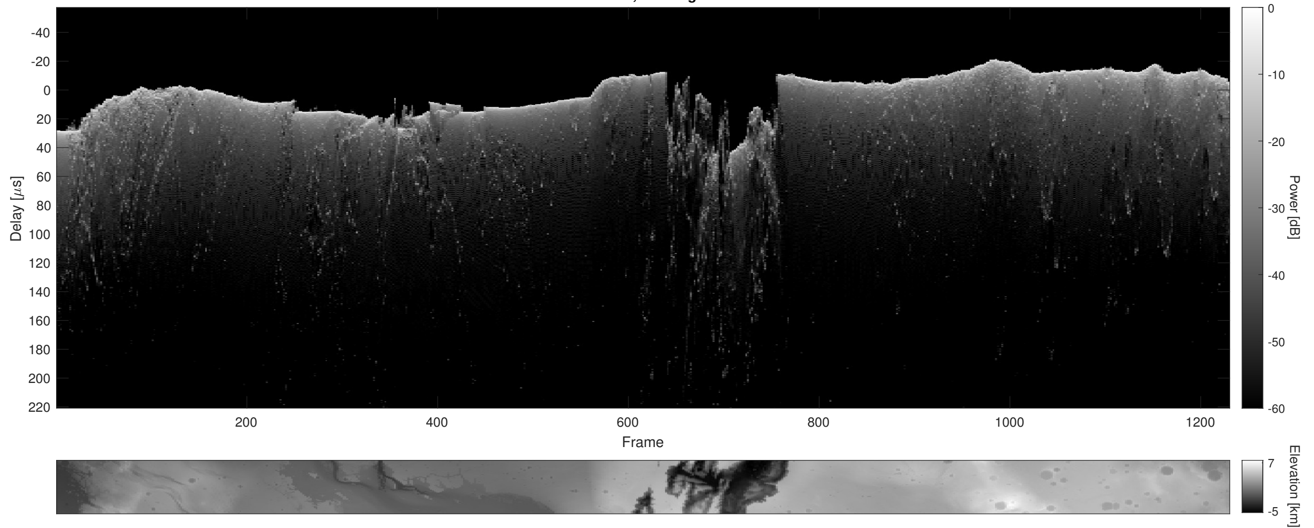
Orbit 5106, Cluttergram
