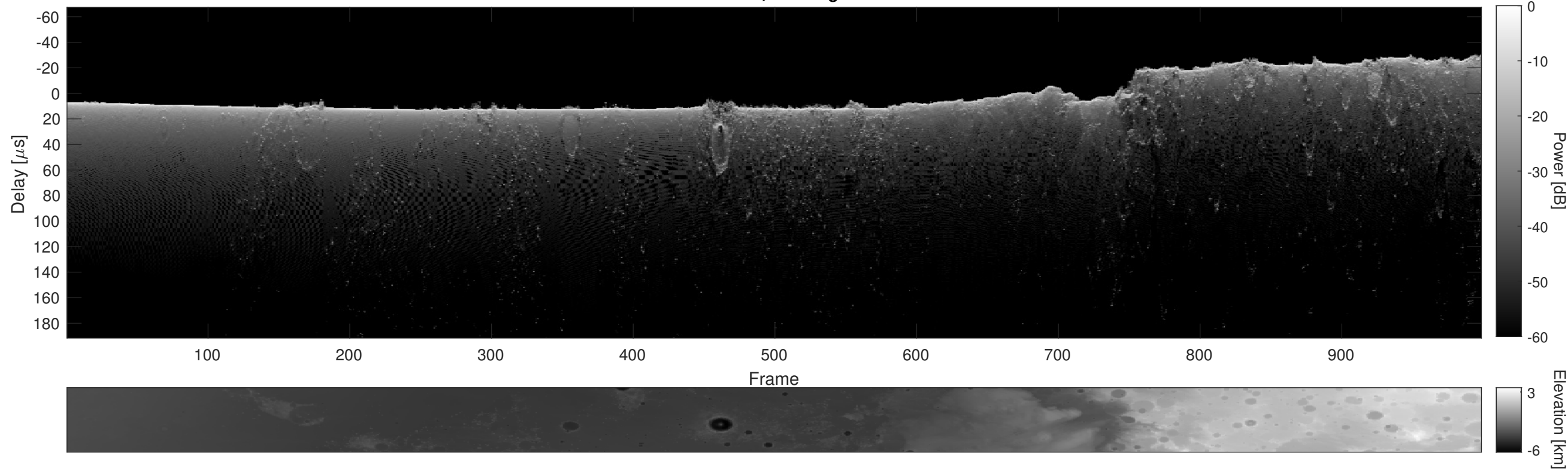
Orbit 5107, Cluttergram
