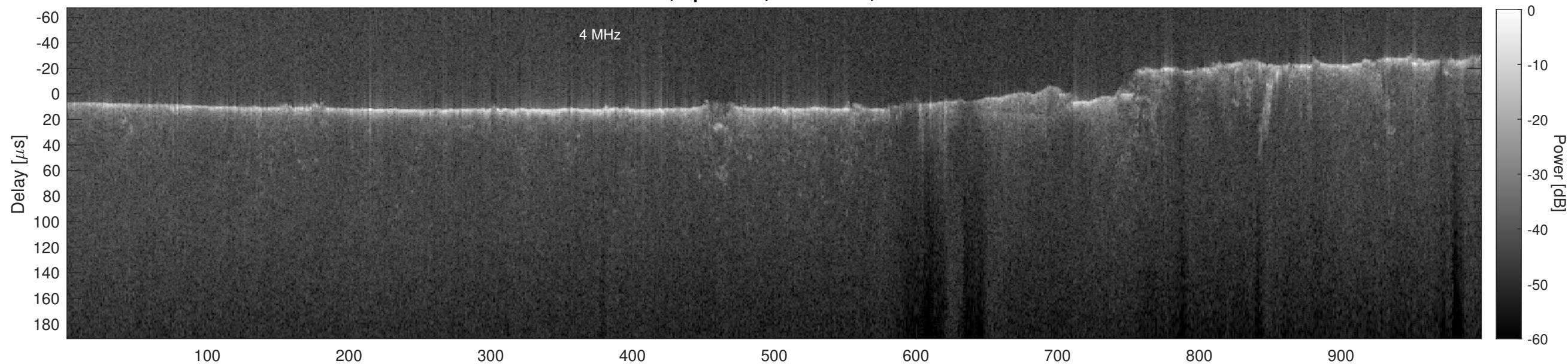
Orbit 5107, Cluttergram
