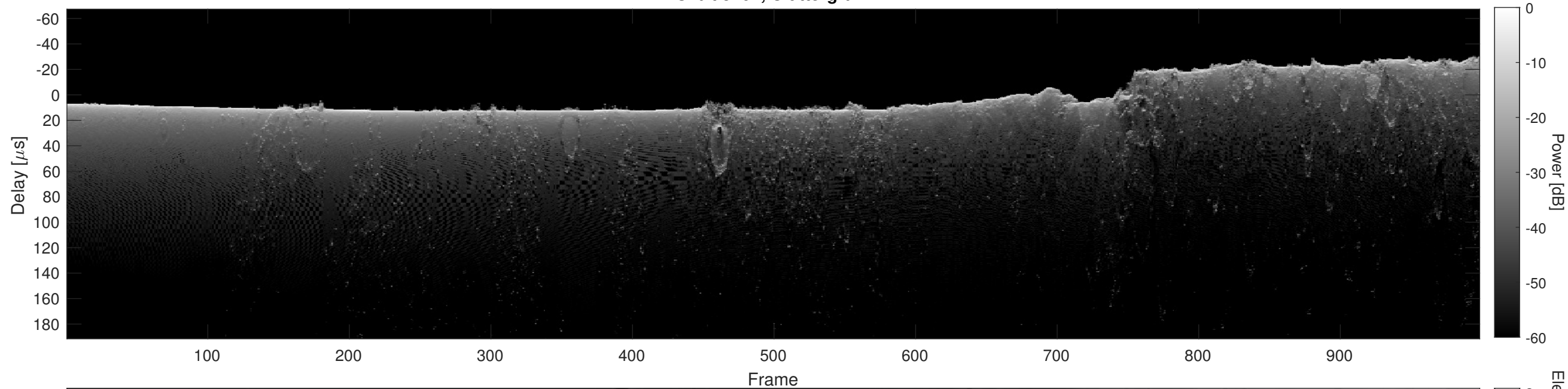
Orbit 5107, Cluttergram
