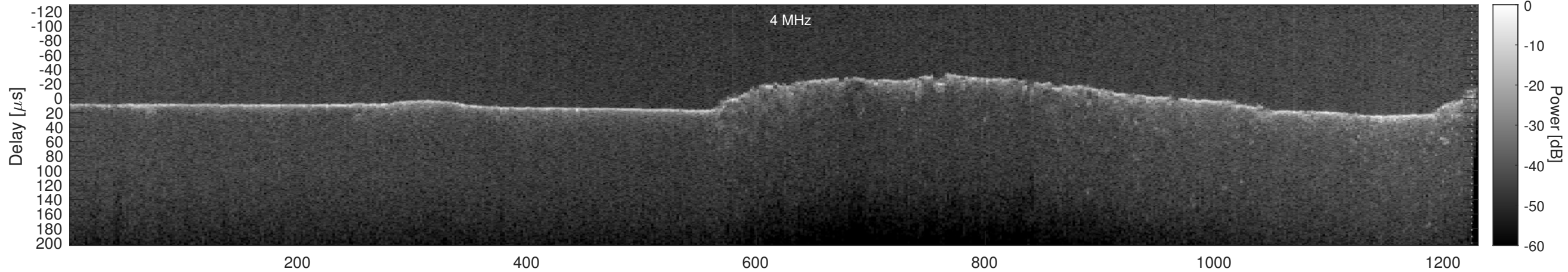
Orbit 5108, Cluttergram
