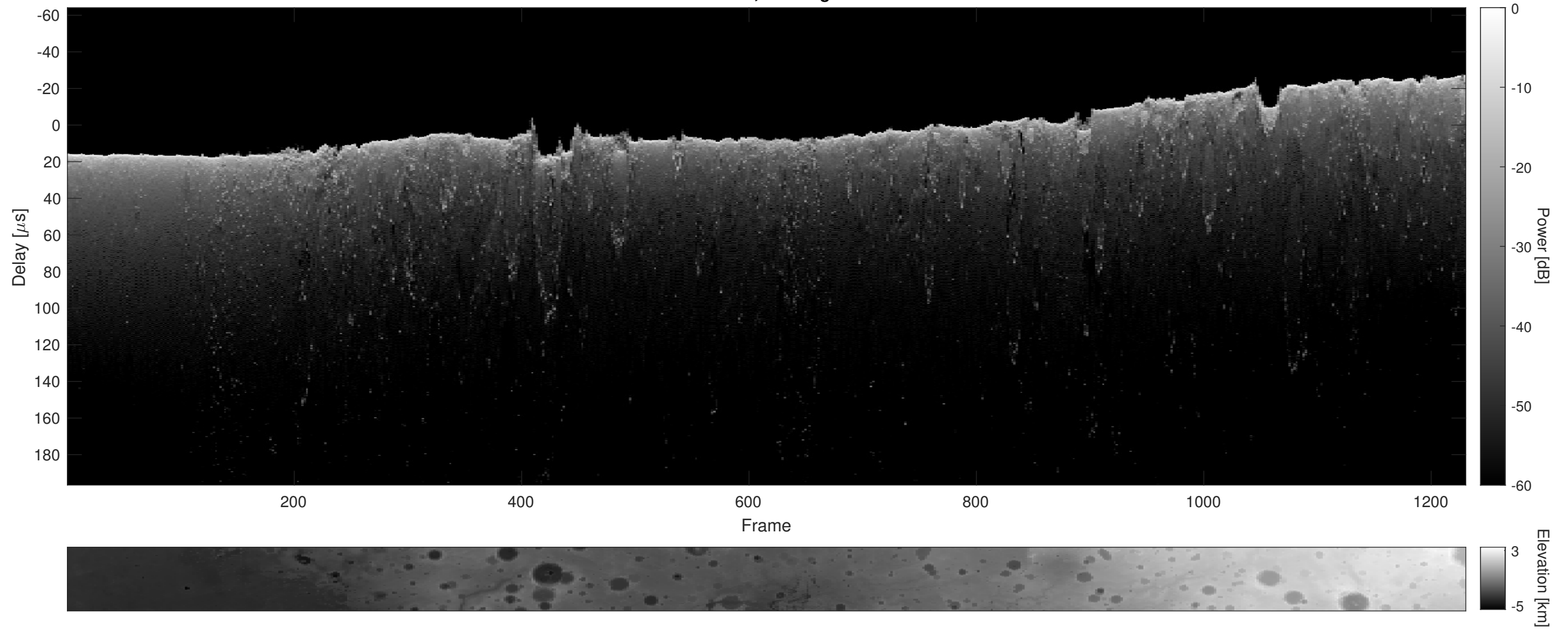
Orbit 5109, Cluttergram
