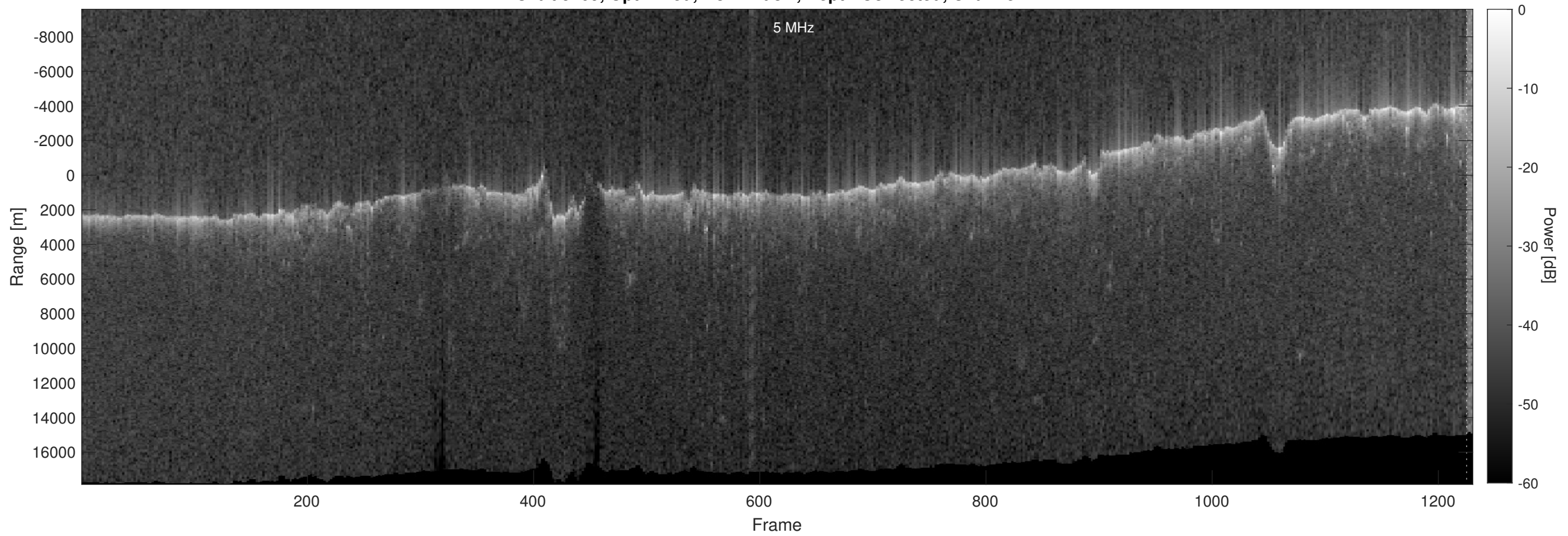
Orbit 5109, Optimized, No Window, Depth-Corrected, Channel 2
