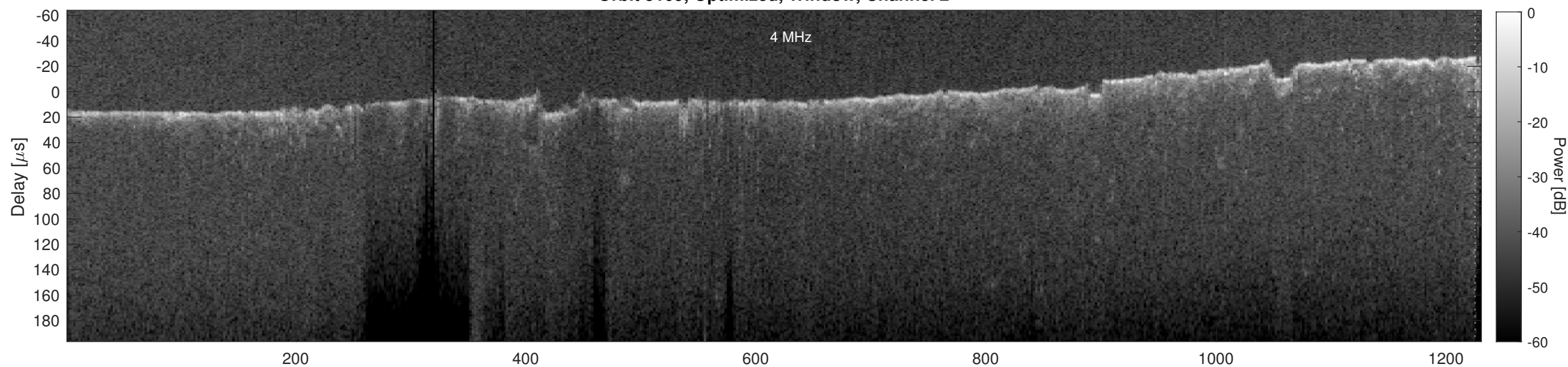
Orbit 5109, Cluttergram
