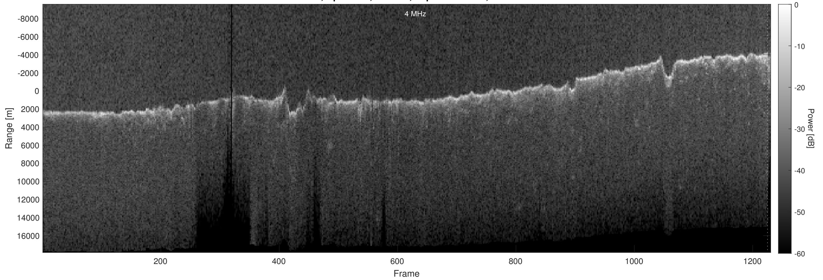
Orbit 5109, Optimized, Window, Depth-Corrected, Channel 2
