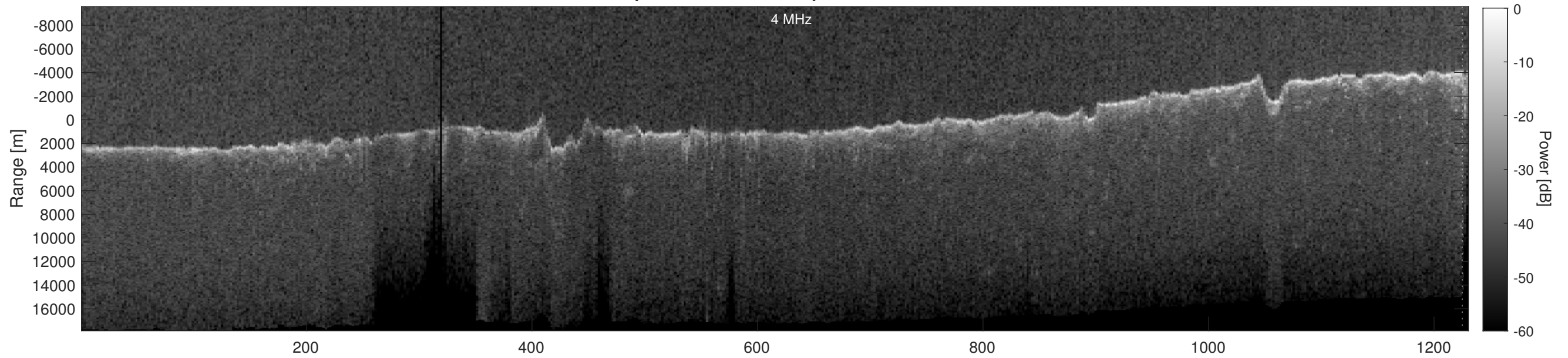
Orbit 5109, Depth-Corrected Cluttergram
