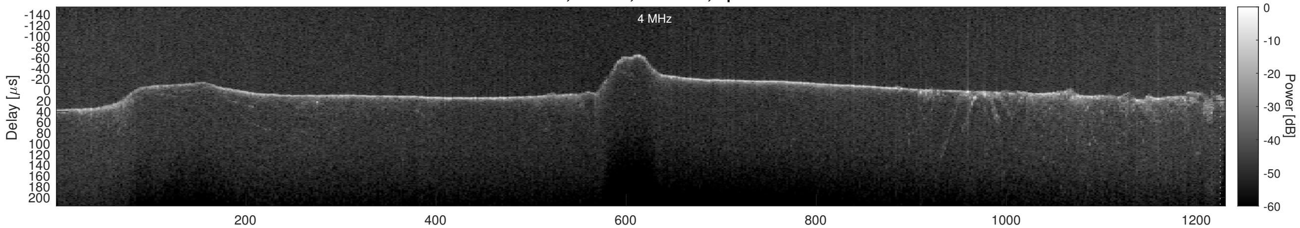
Orbit 5110, Cluttergram
