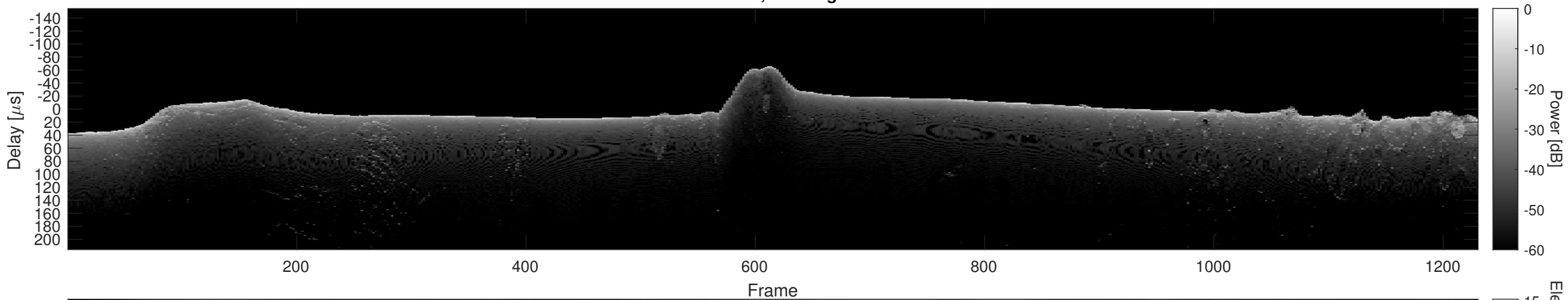
Orbit 5110, Cluttergram
